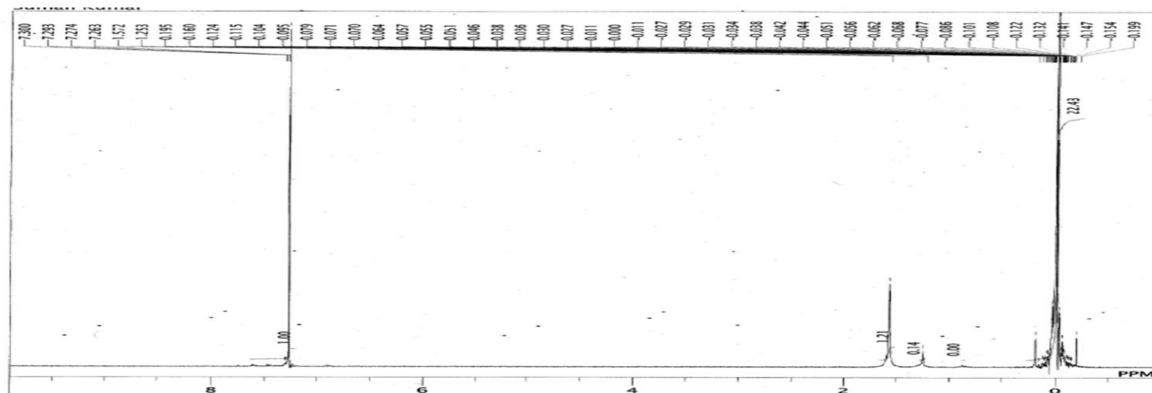
Fig. D: Superimposed IR spectra of standard quercetin and isolated quercetin
