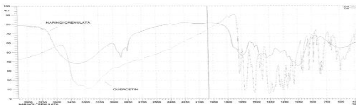
Fig. D: Superimposed IR spectra of standard quercetin and isolated quercetin
