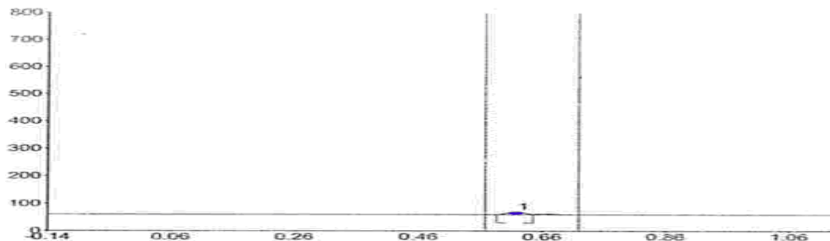
Fig. C: HPTLC chromatogram of quercetin from callus extract
